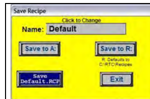
Fig 4-2a Save Recipe
