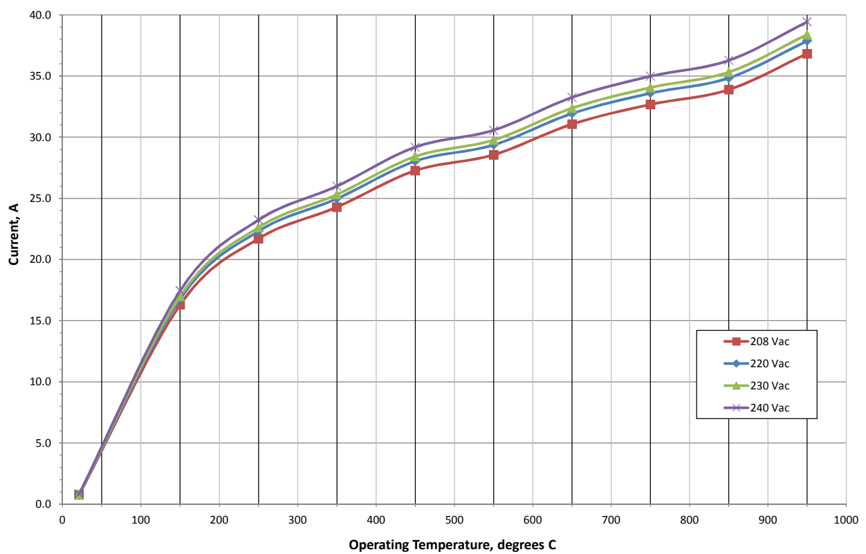
Standard LA-306 Average Current at Operating Temperatures
